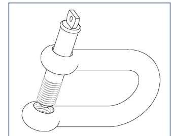
S6733 8mm D Shackle Galv. S5382 10mm D Shackle Galv.
