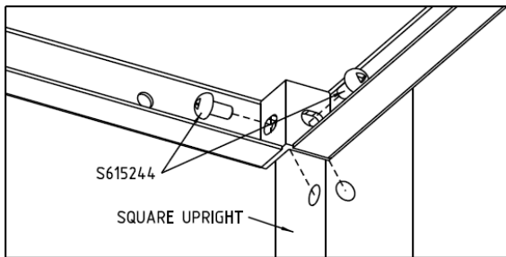
ALY AND TIMBER PLATFORMS S615244 TRILOBE 10x20
