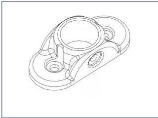
S7749 Flange (48.3mm O.D.) S7751 Flange (42.4mm O.D.) S7753 Flange (33.7mm O.D.)
