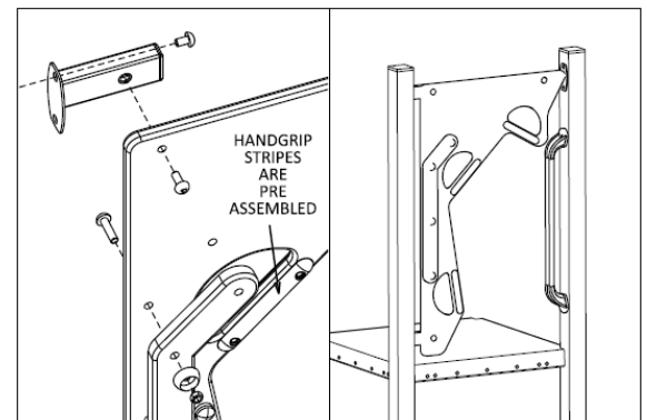
6. Entrance Panel Offset
