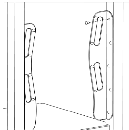
1. Access Panel
