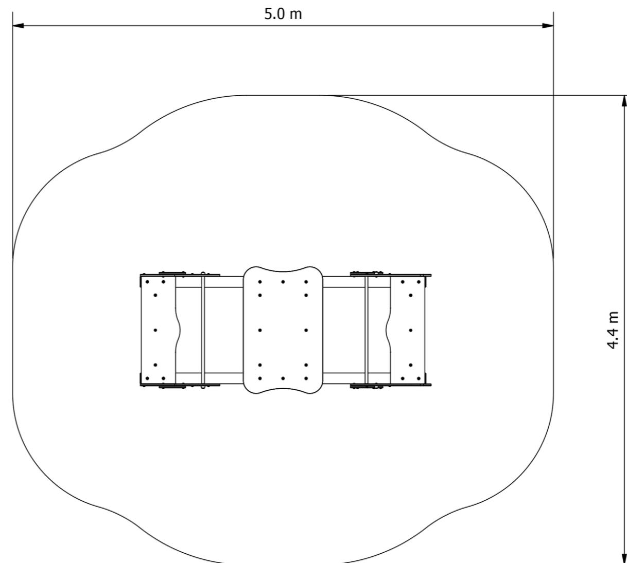
Plan View
