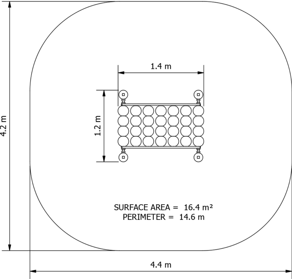
Plan View
