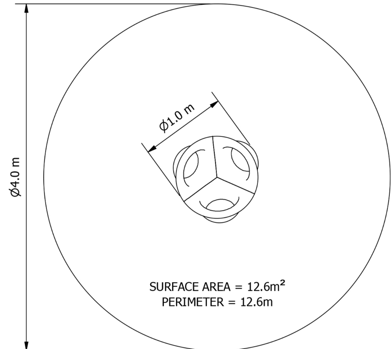
Plan View
