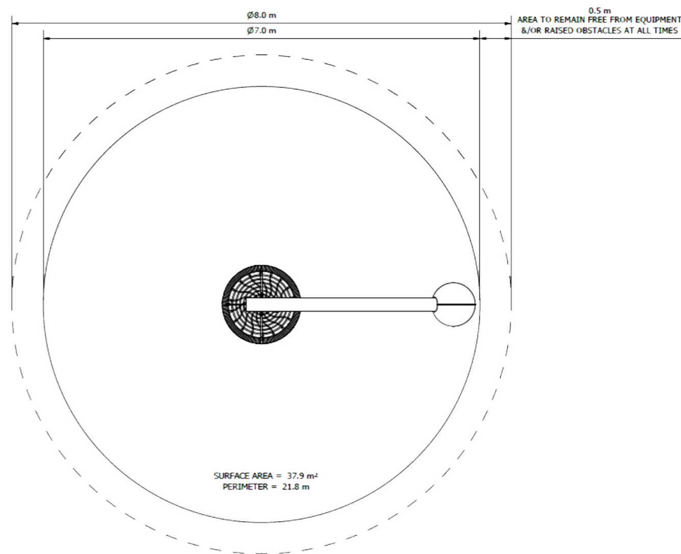
Plan View
