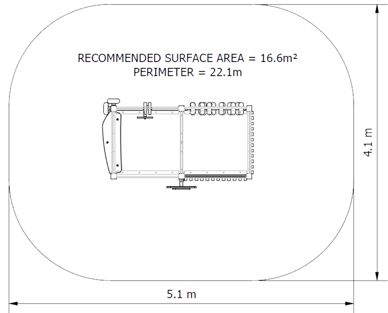
Plan View
