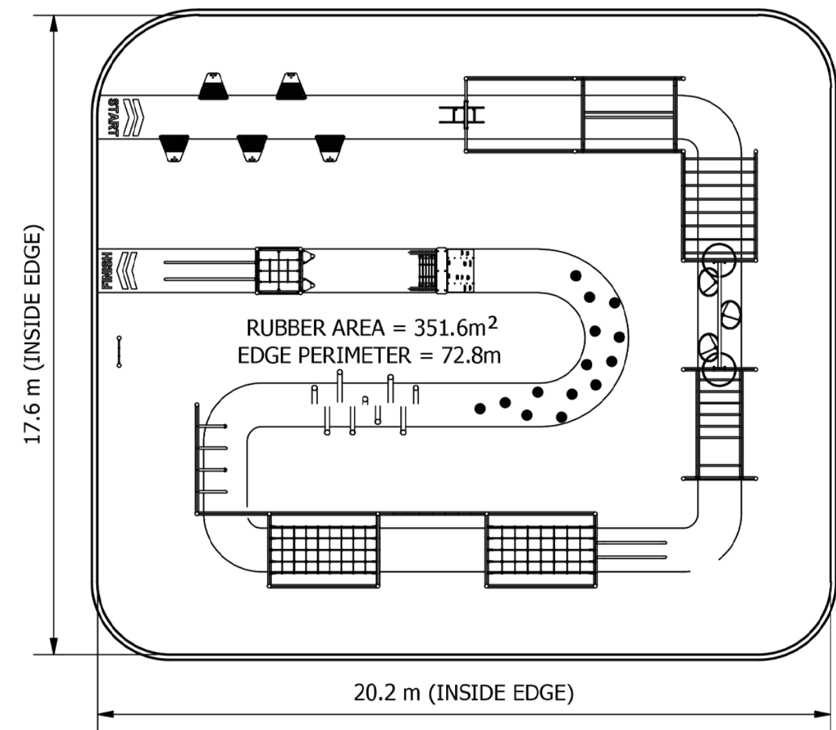
Plan View
