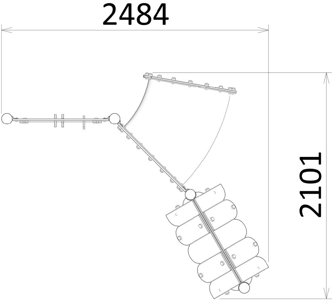
Plan View
