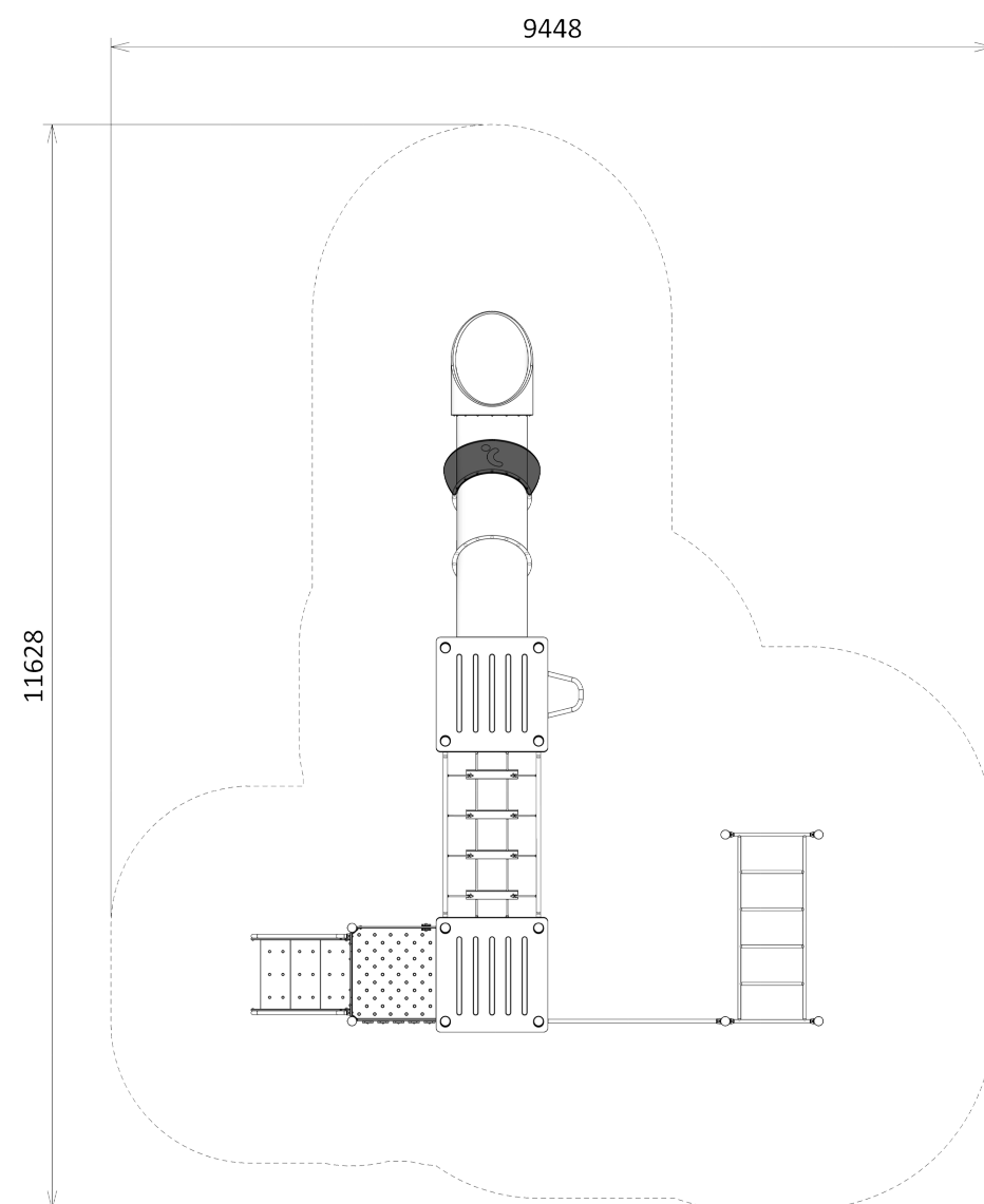
Plan View
